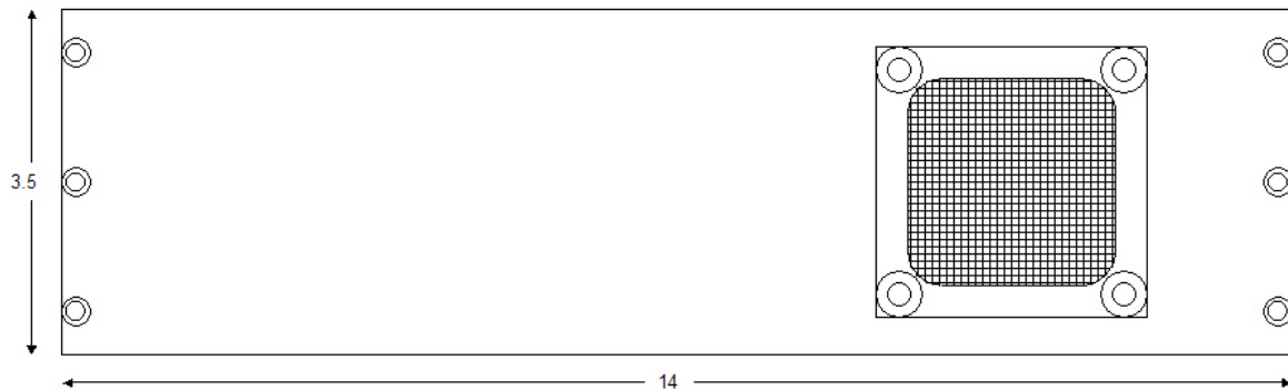
SIDE VIEW
