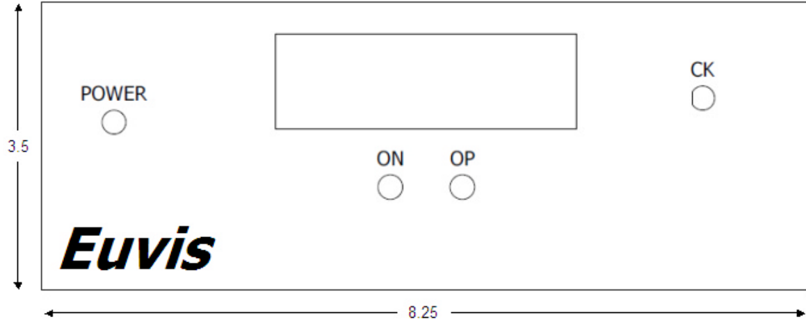
FRONT VIEW
